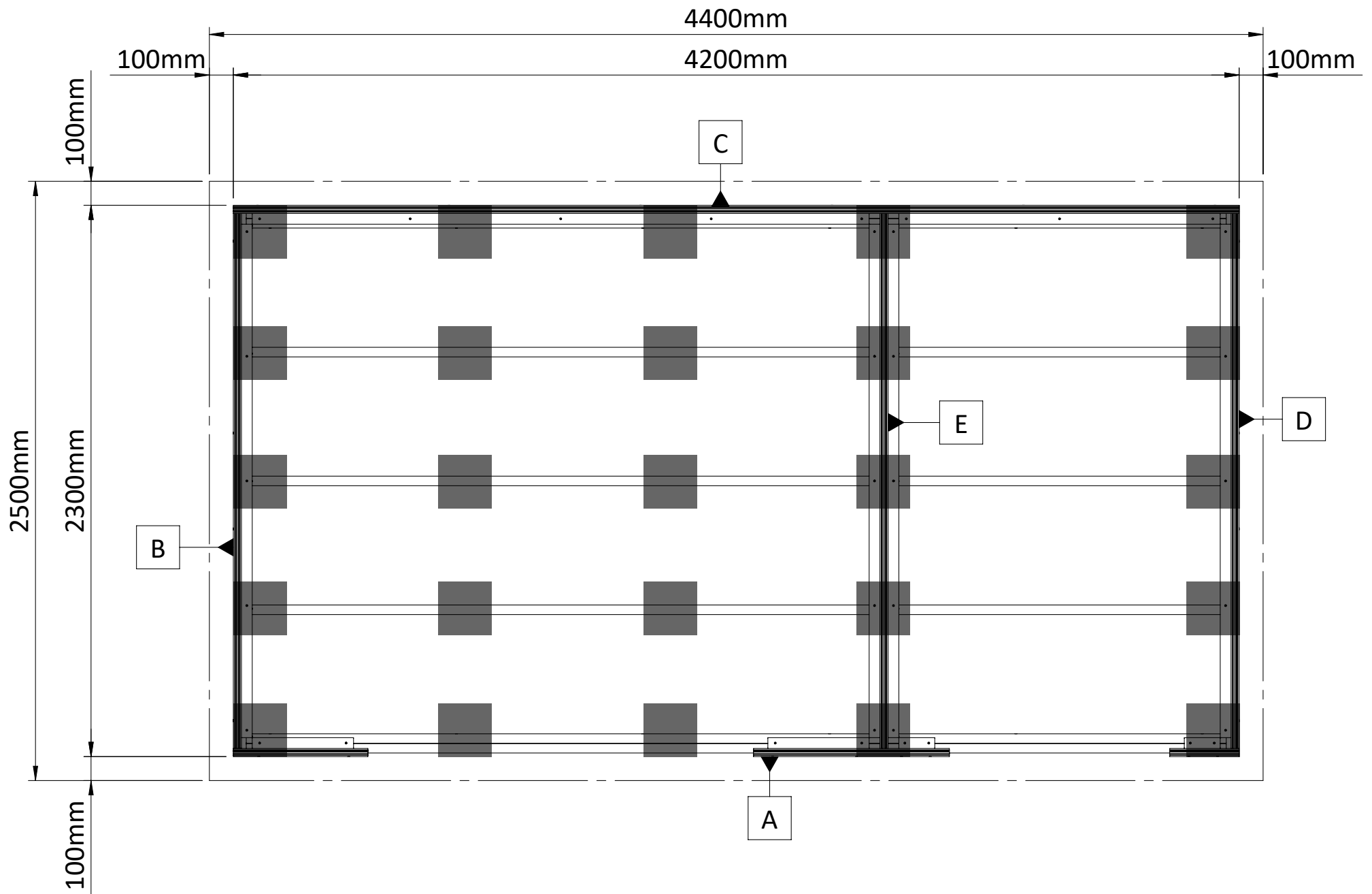
PLINTPLAN / FOUNDATION PLAN / BETONBLOCK / PLAN DE FONDATIONS
