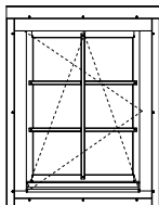
Single window db. gl 2 st. 70 mm 765 x 990 mm
