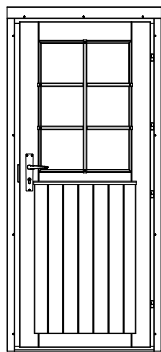
Single Door db. gl 2 st. 70 mm L+R 840 x 1955 mm +12 mm
