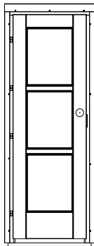
Single Door tempered gl. 1 st. 70 mm 840 x 1955 mm +12 mm
